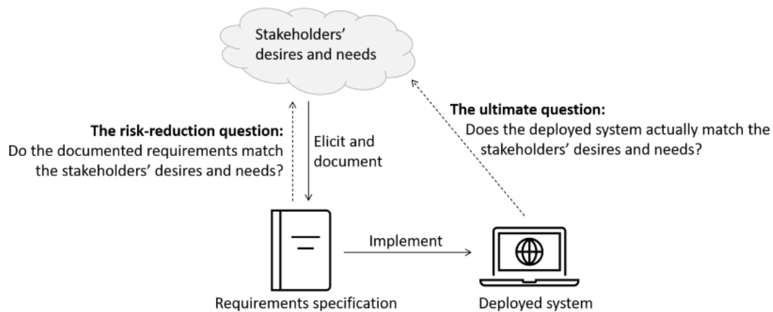
Figure 2.4 Validation [Glin2019]
