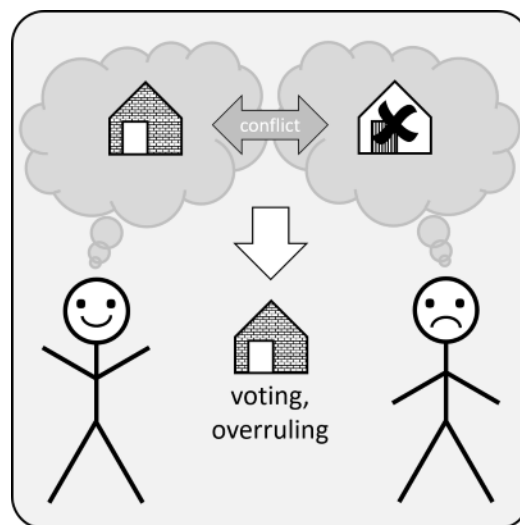
Figure 4.12 Voting
